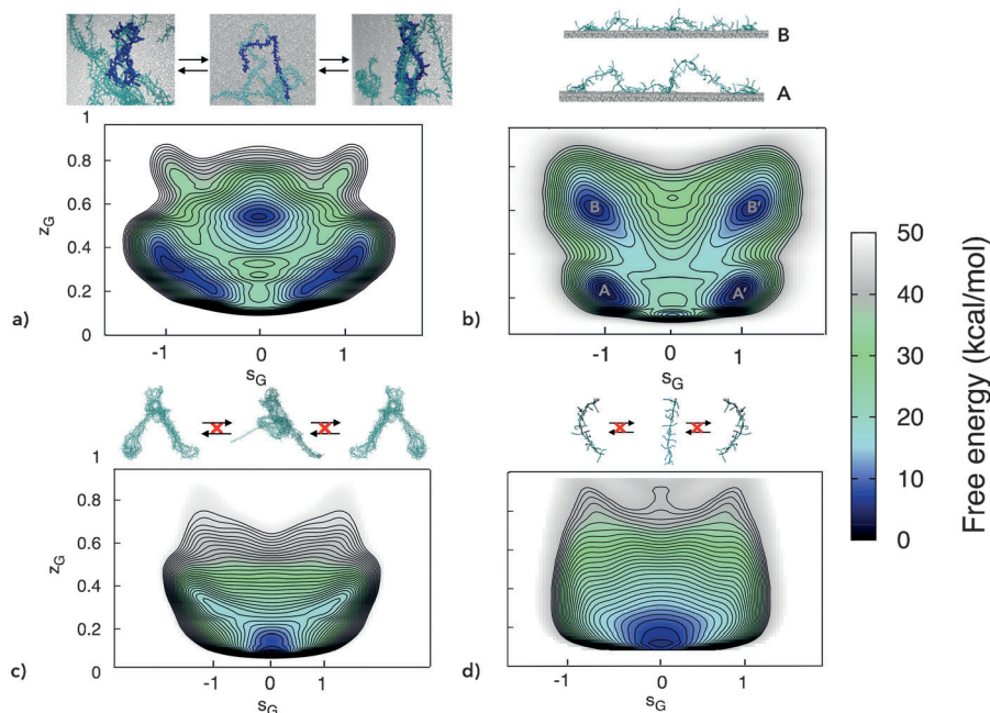
Figure 1. Free-energy profiles of the achiral-to-chiral transition of PDOF. a) Sixteen chains of PDOF deposited on amorphous silica (top: chain models corresponding to the chiral switch cycle), b) one chain of PDOF deposited on amorphous silica (top: the anchoring of PDOF on amorphous silica (A and B), c) sixteen chains of PDOF in vacuum, and d) one chain of PDOF in vacuum. In (a), where the chiral cycle can occur, the free-energy basins in the main panel correspond to the models shown in deep blue. A picture of the forbidden transition is also shown in (c) and (d).
